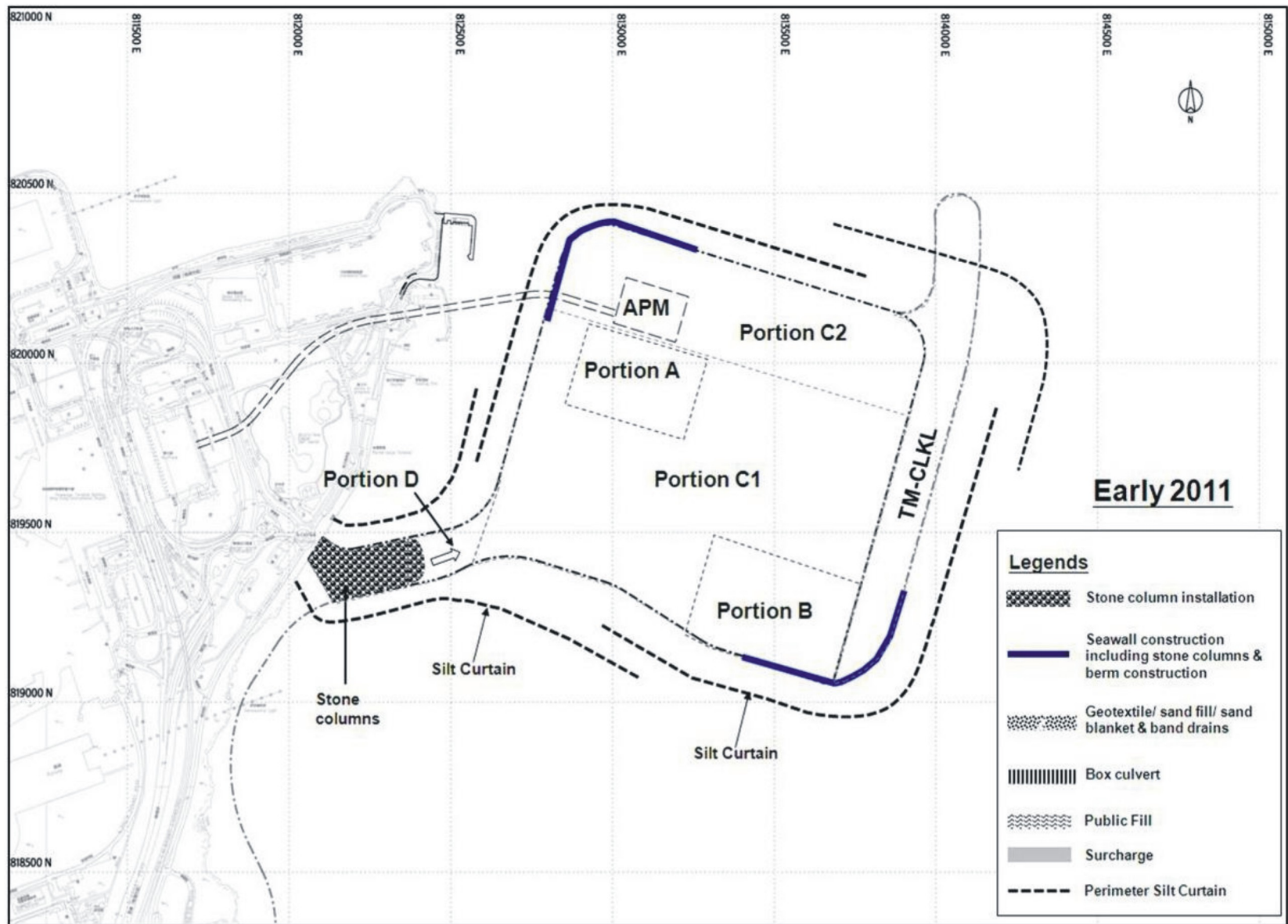
Figure 12 - Outline of Construction Sequence (Sheet 1 of 10) 圖 12 - 施工程序大綱(表10之1)
